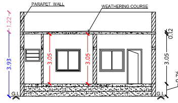
Section on-"AA"
