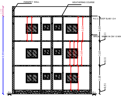
Section on-"AA"
