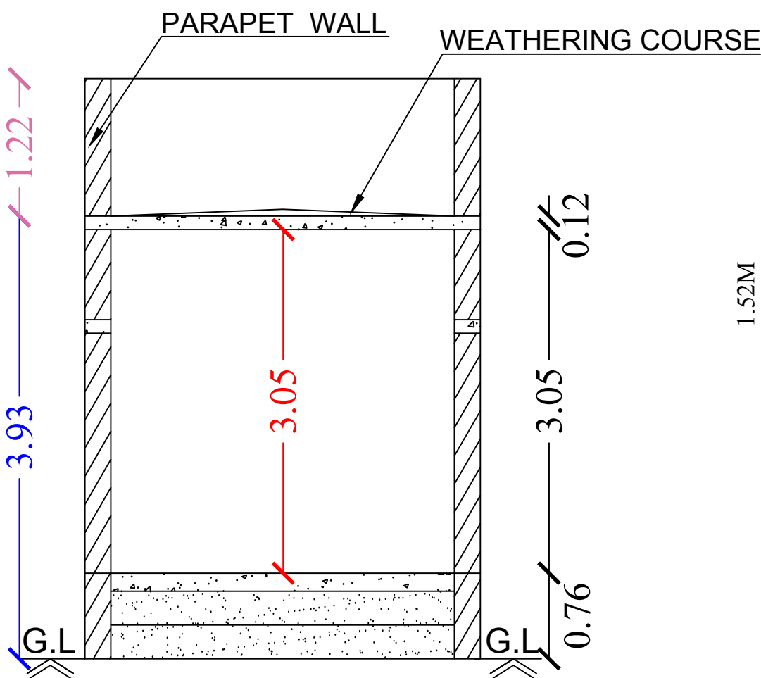
Section on-"AA"
