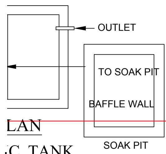
SEPTIC TANK
