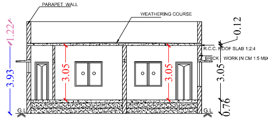
Section on-"AA"
