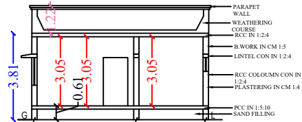
SECTION ON R.P.
