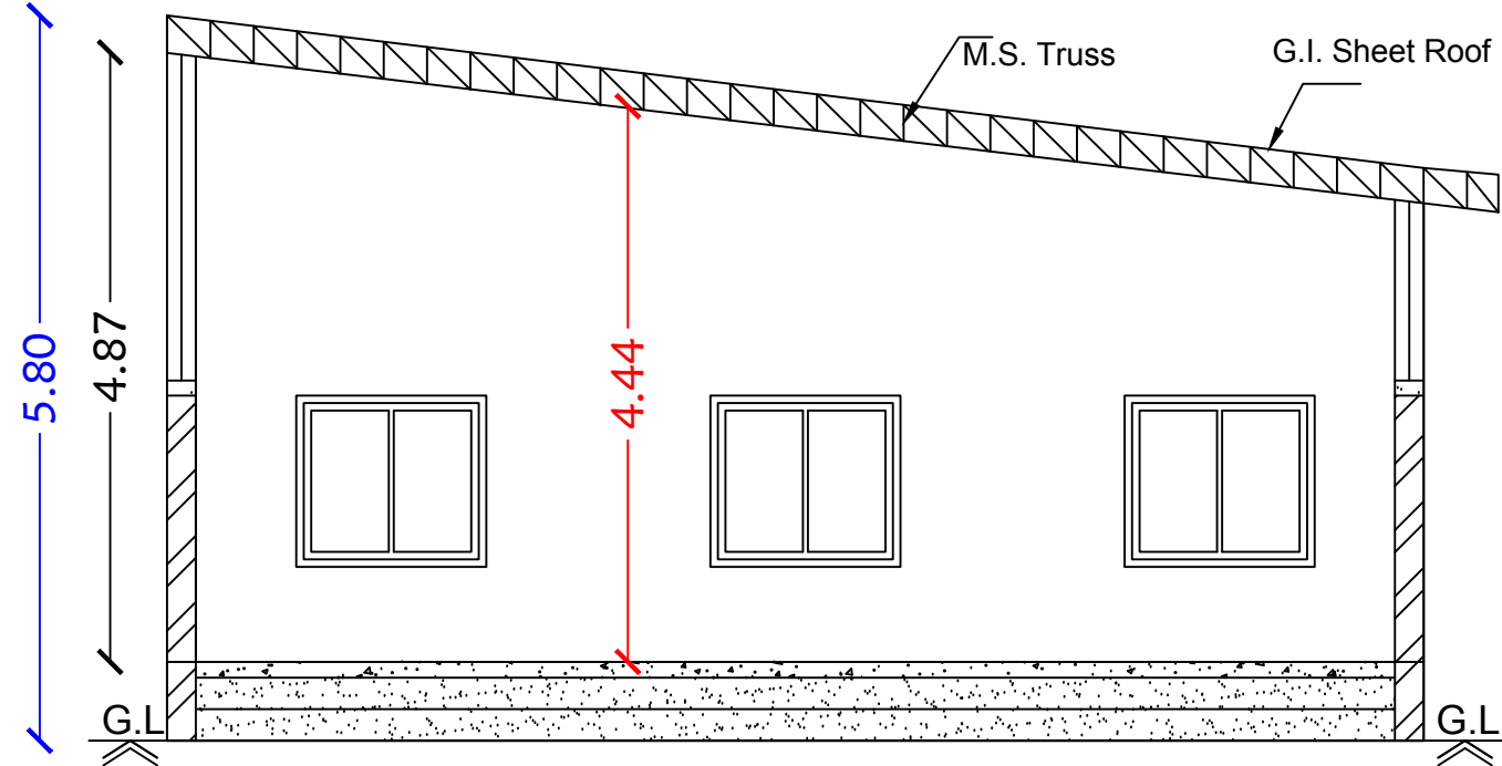
Section on-"AA"
