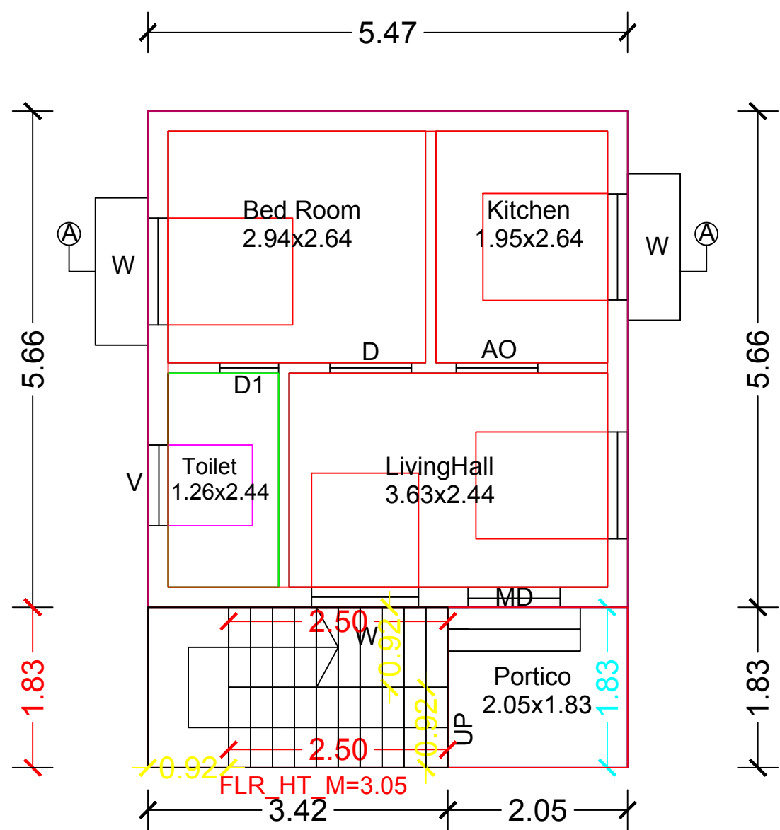
Ground Floor
