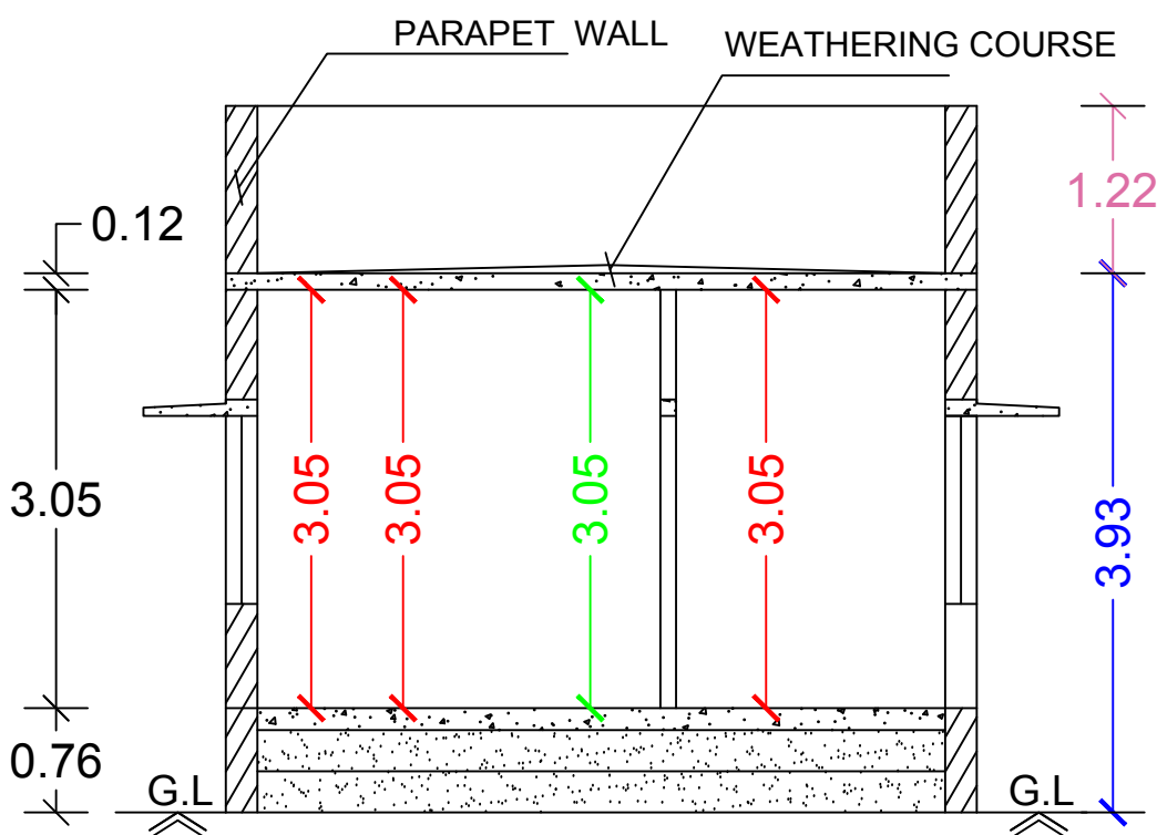
Section on-"AA"
