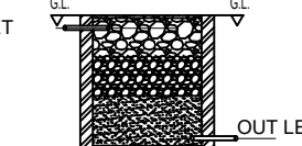
RAINWATER STORAGE PIT DETAILS
