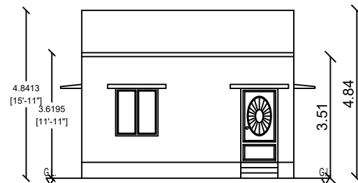
ELEVATION ON EAST
