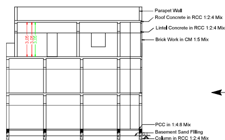
Section RR
