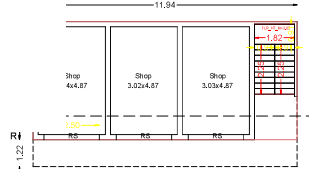
Existing Ground Floor Plan
