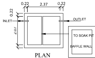
PLAN SEPTIC TANK
