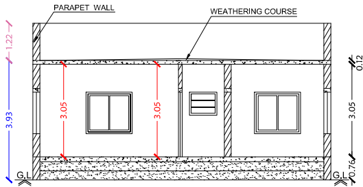
Section on-"AA"
