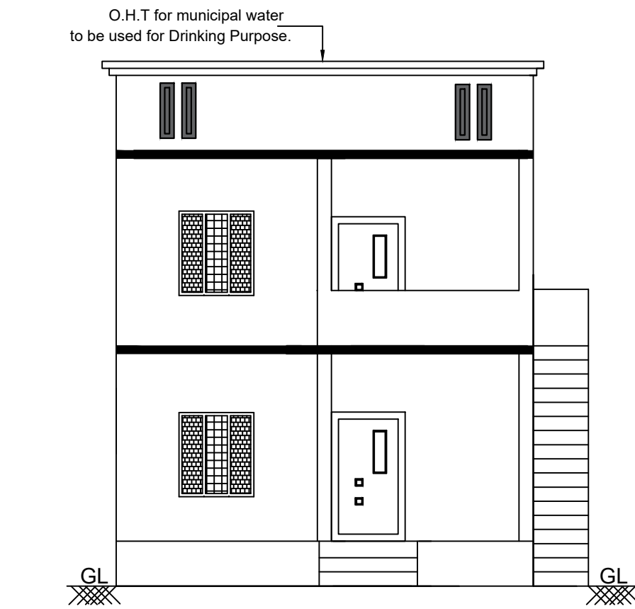
FRONT ELEVATION
