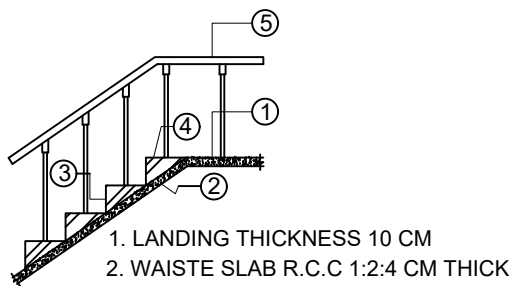
Staircase Details
