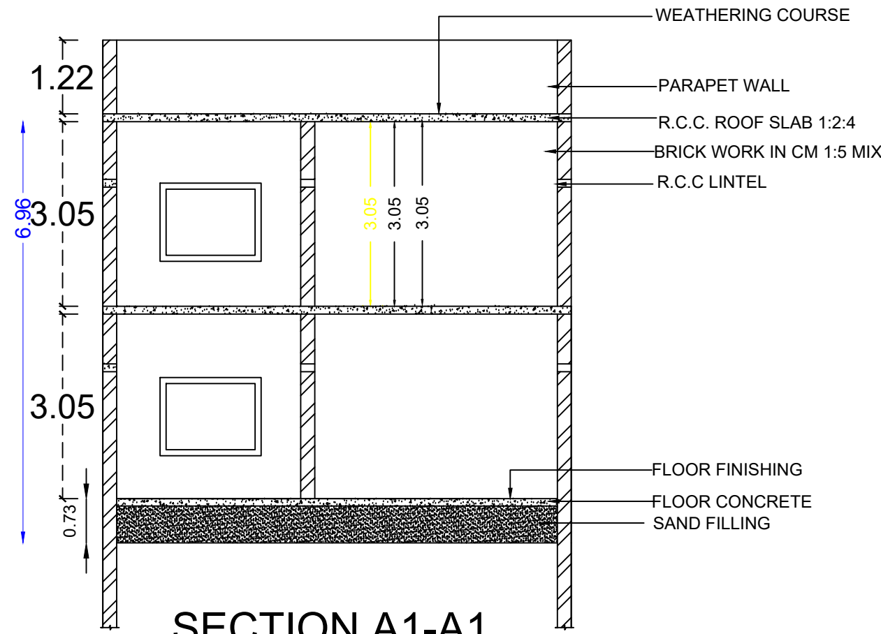
SECTION A1-A1
