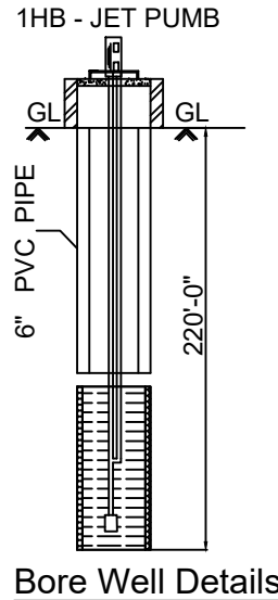
Bore Well Details
