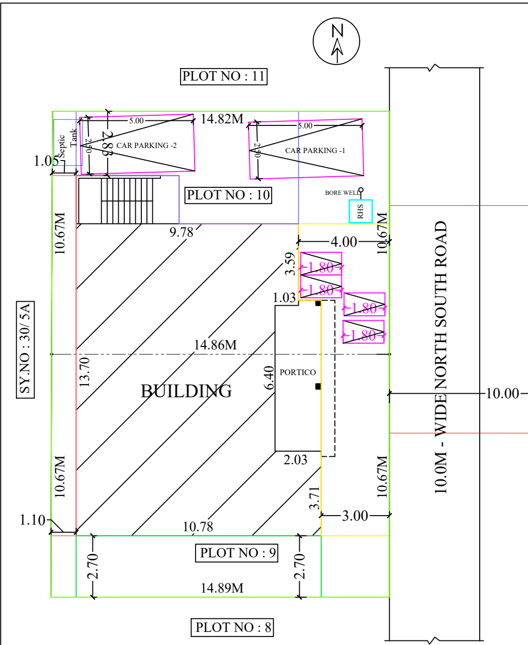
SITE PLAN (1:100)
