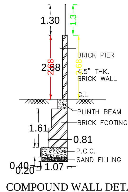
COMPOUND WALL DETAILS
