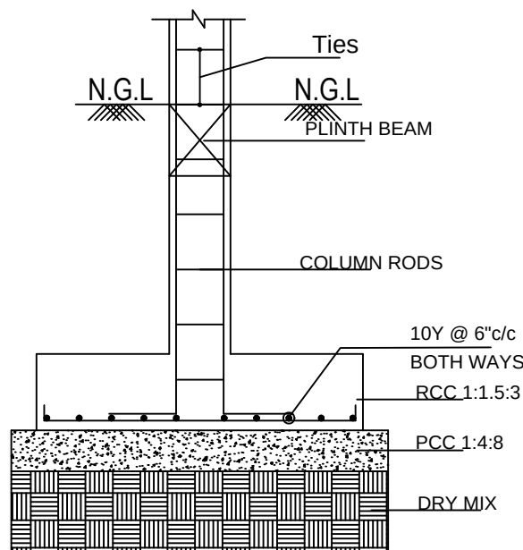
FOUNDATION DETAILS (Concentric Footing)
