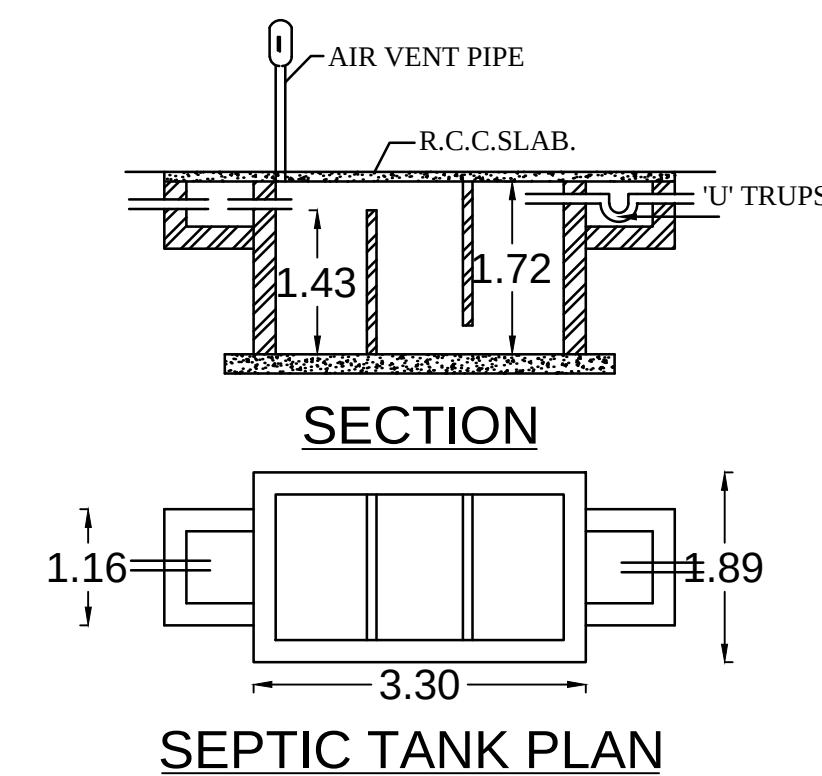
SEPTIC TANK PLAN
