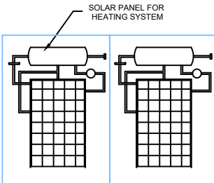
SOLAR HEATING SYSTEM
