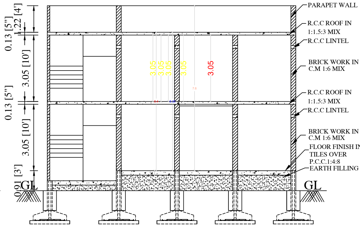
SECTION AA
