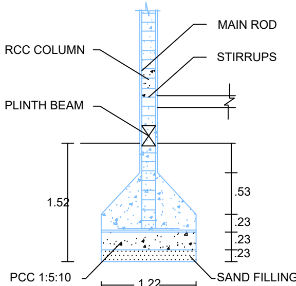
COLUMN DETAILS
