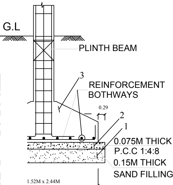
COLUMN FOOTING
