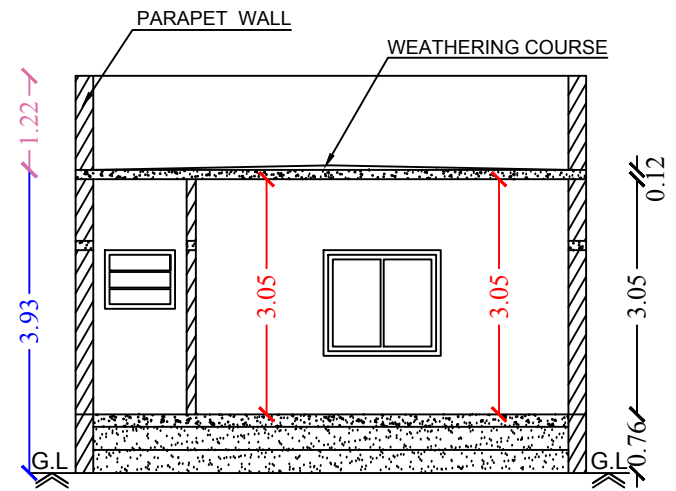
Section on-"AA"
