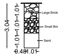
SECTION OF RAIN WATER COLLECTION PITS (NTS)
