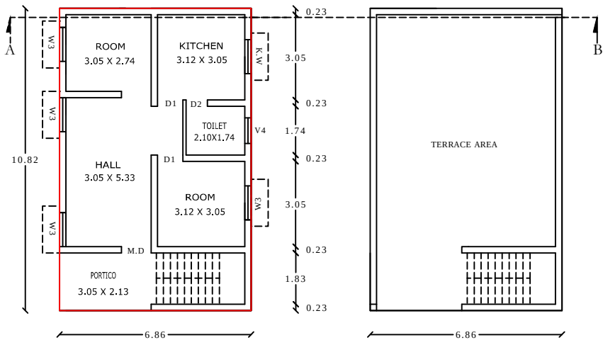
TERRACE FLOOR
