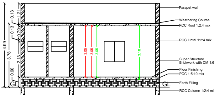
SECTION ON "VR"
