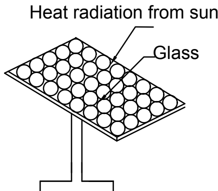
SOLAR SYSTEM (Scale 1:100)
