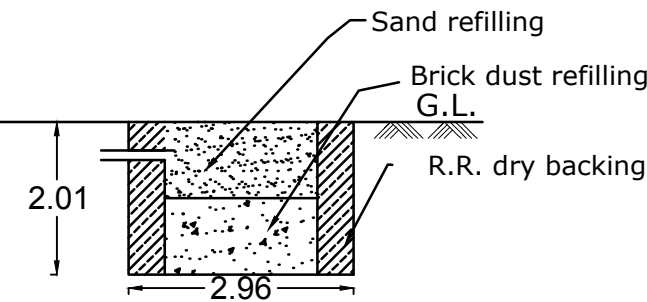
DETAILS OF RAIN WATER HARVESTING
