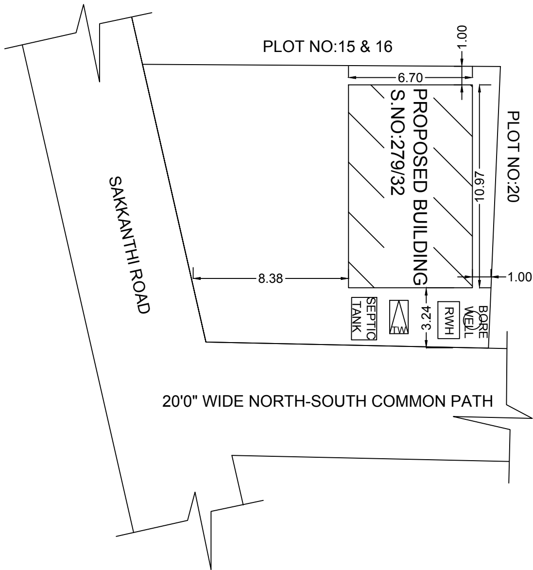
SITE PLAN
