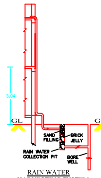
RAIN WATER HARVESTING SYSTEM RW_HCAPACITY_L=1000LTRS
