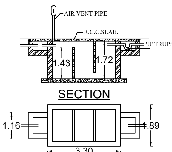
SECTION SEPTIC TANK PLAN
