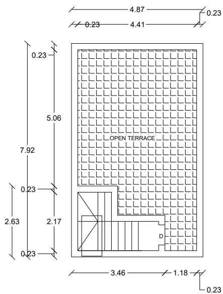
TERRACE FLOOR
