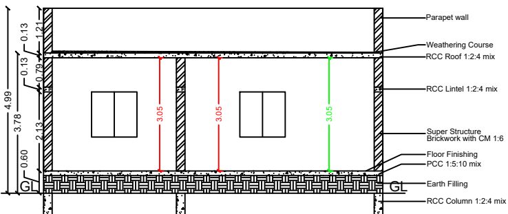
SECTION ON "VR"
