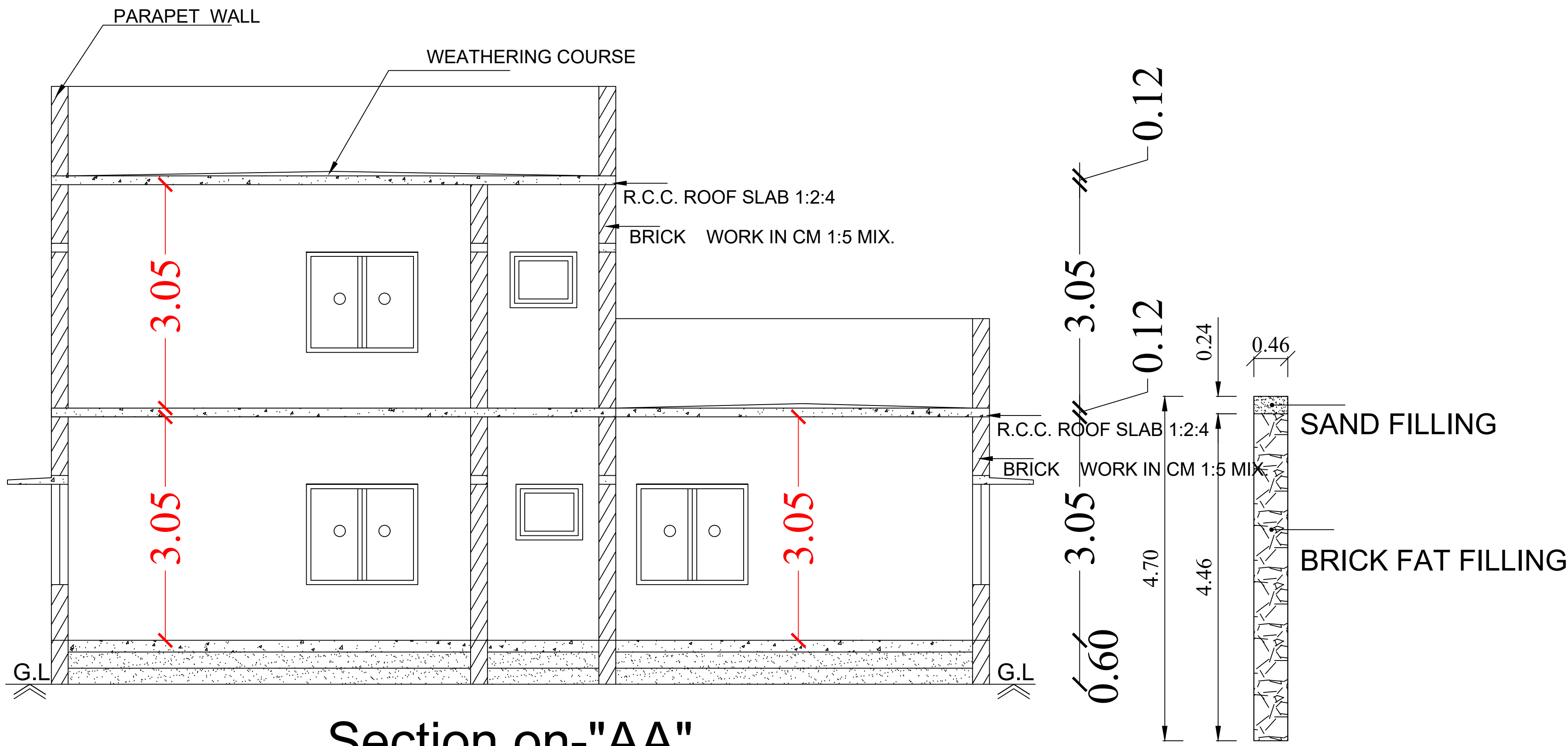
Section on-"AA"
