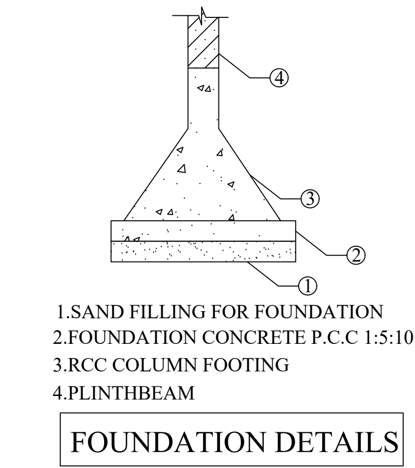
FOUNDATION DETAILS
