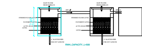
CUT SECTION ON AA
