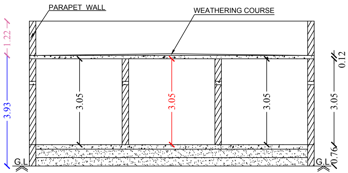
Section on-"AA"
