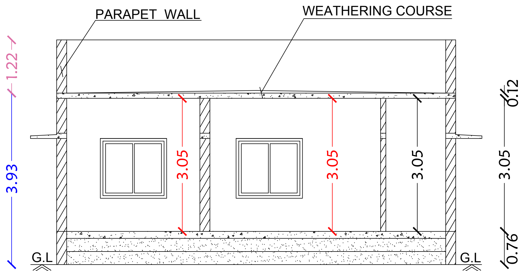
Section on-"AA"
