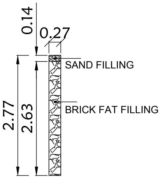
DETAILS OF PERCUATION PIT
