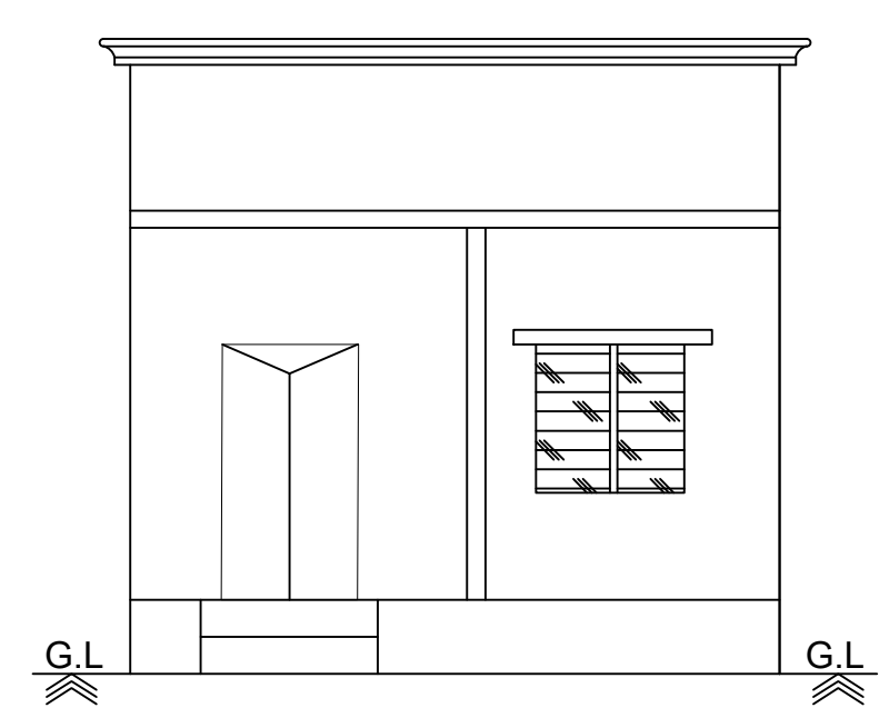
FRONT ELEVATION
