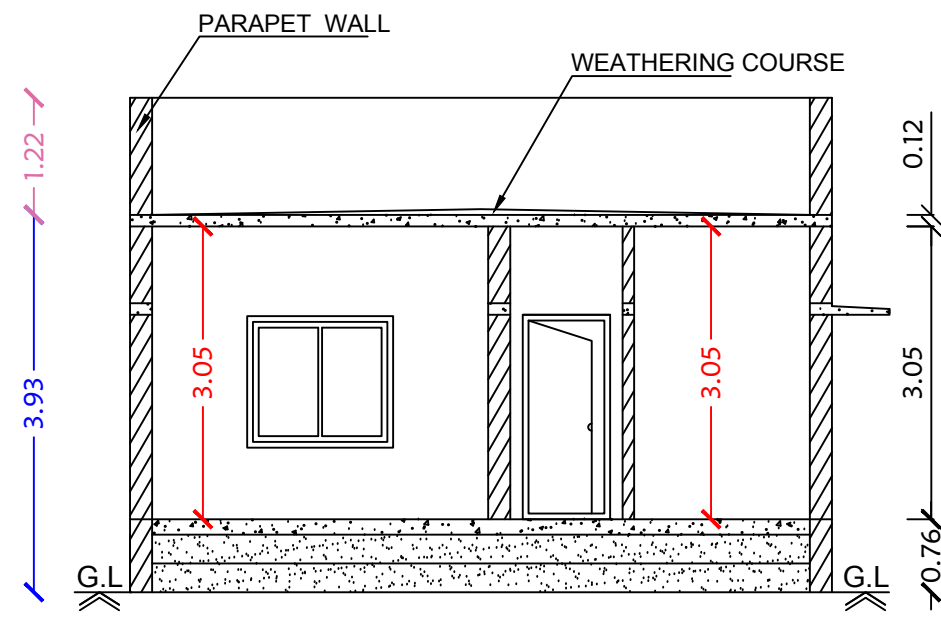
Section on-"AA"
