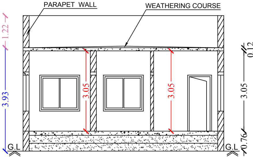
Section on-"AA"
