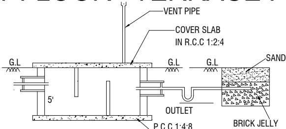
SECTION-AB
