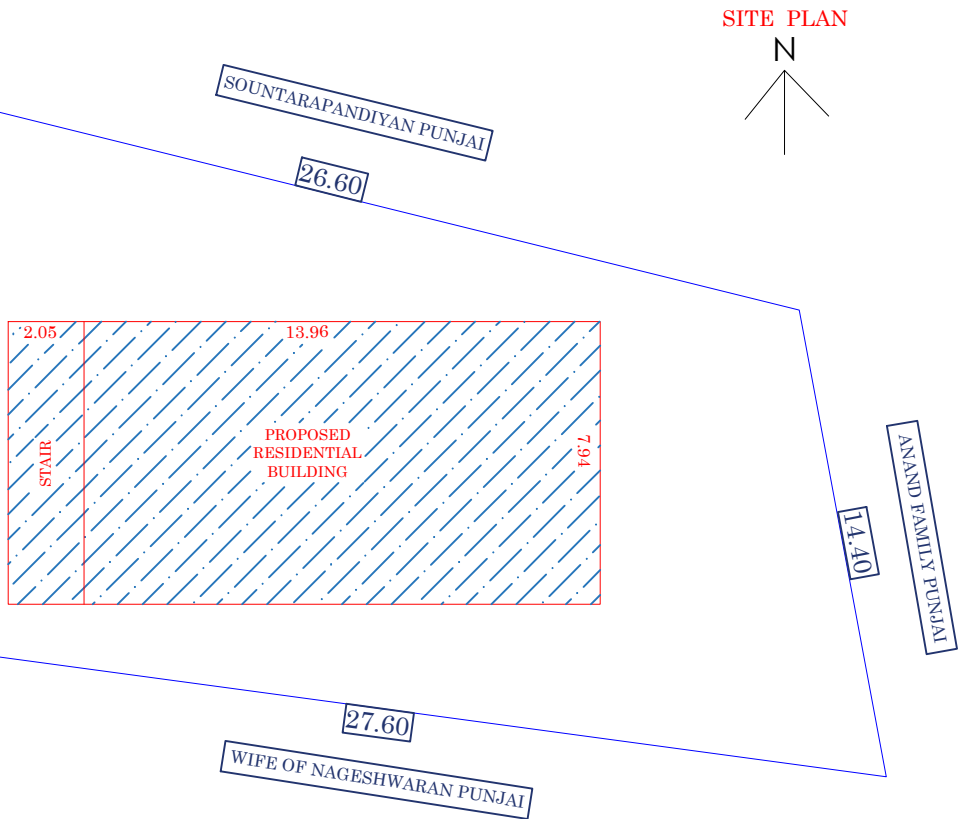
SITE PLAN
