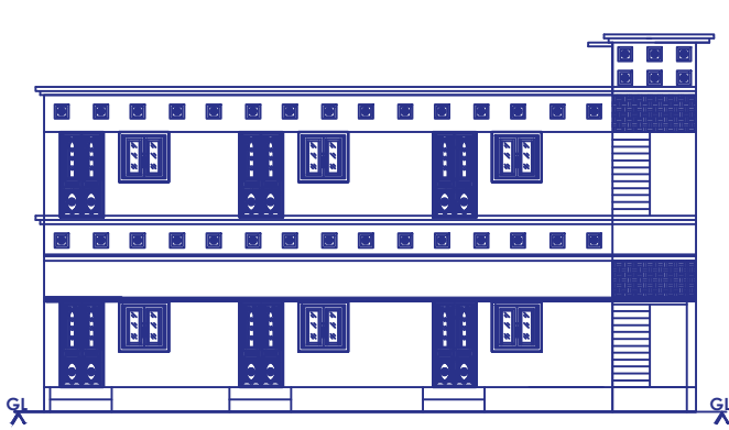
FRONT ELEVATION
