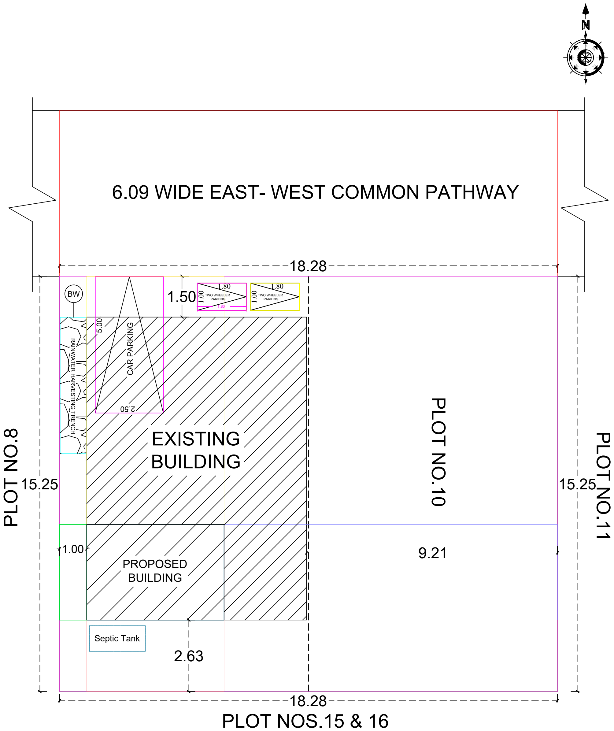
SITE PLAN (1:100)
