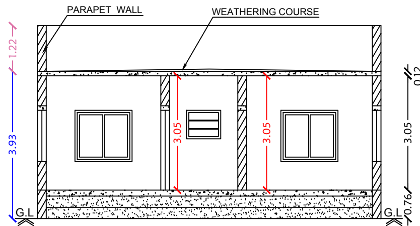
Section on-"AA"
