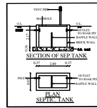
SECTION OF SEPTIC TANK
