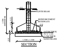
FOUNDATION DETAILS
