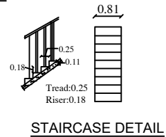
STAIRCASE DETAIL
