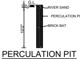
PERCOLATION PIT
