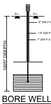
BORE WELL
