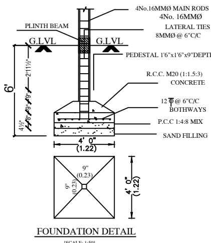
FOUNDATION DETAIL
