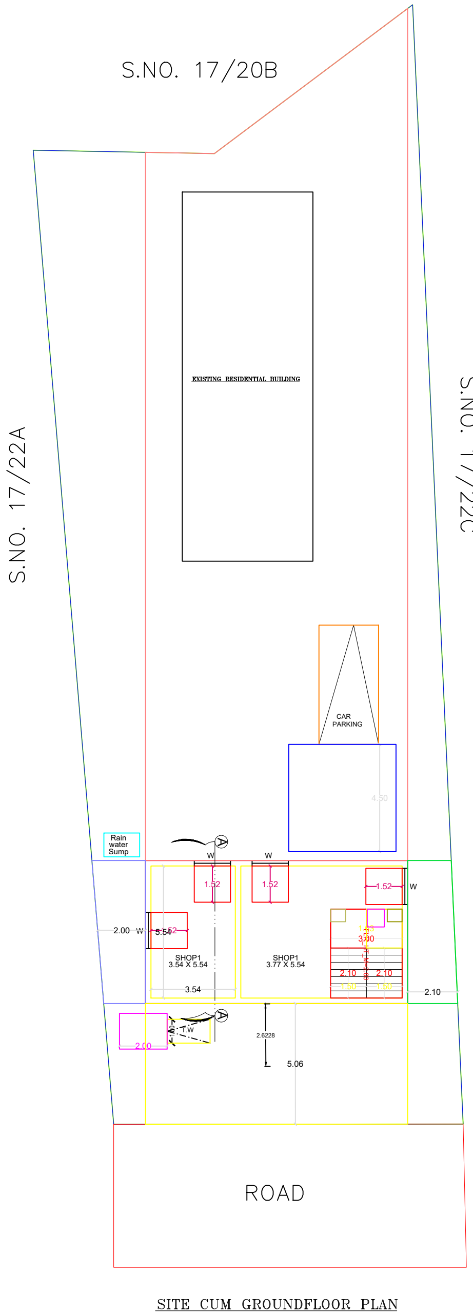
SITE CUM GROUND FLOOR PLAN
