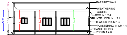
SECTION ON 'RP'
