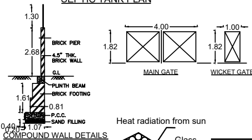
COMPOUND WALL DETAILS
