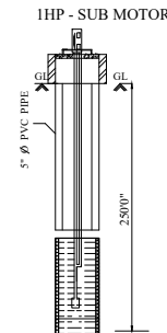
BOREWELL DETAILS
