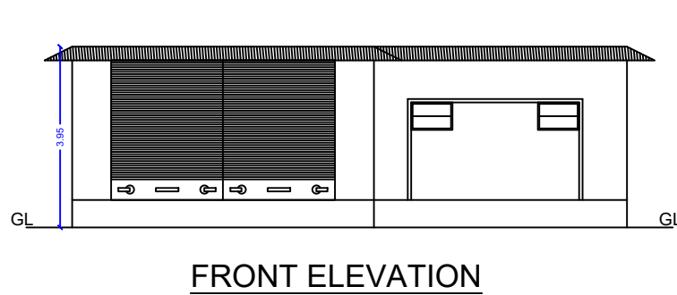
FRONT ELEVATION
