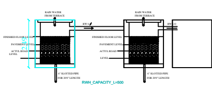
CUT SECTION ON AA
