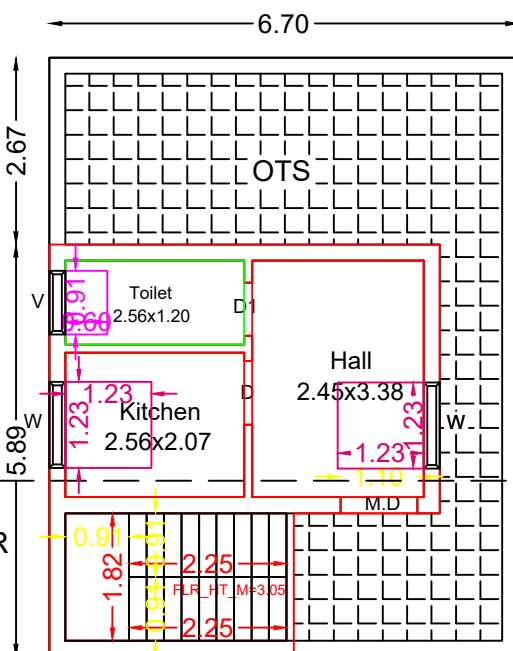
Pro.Second Floor Plan
