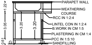
SECTION ON R/P
