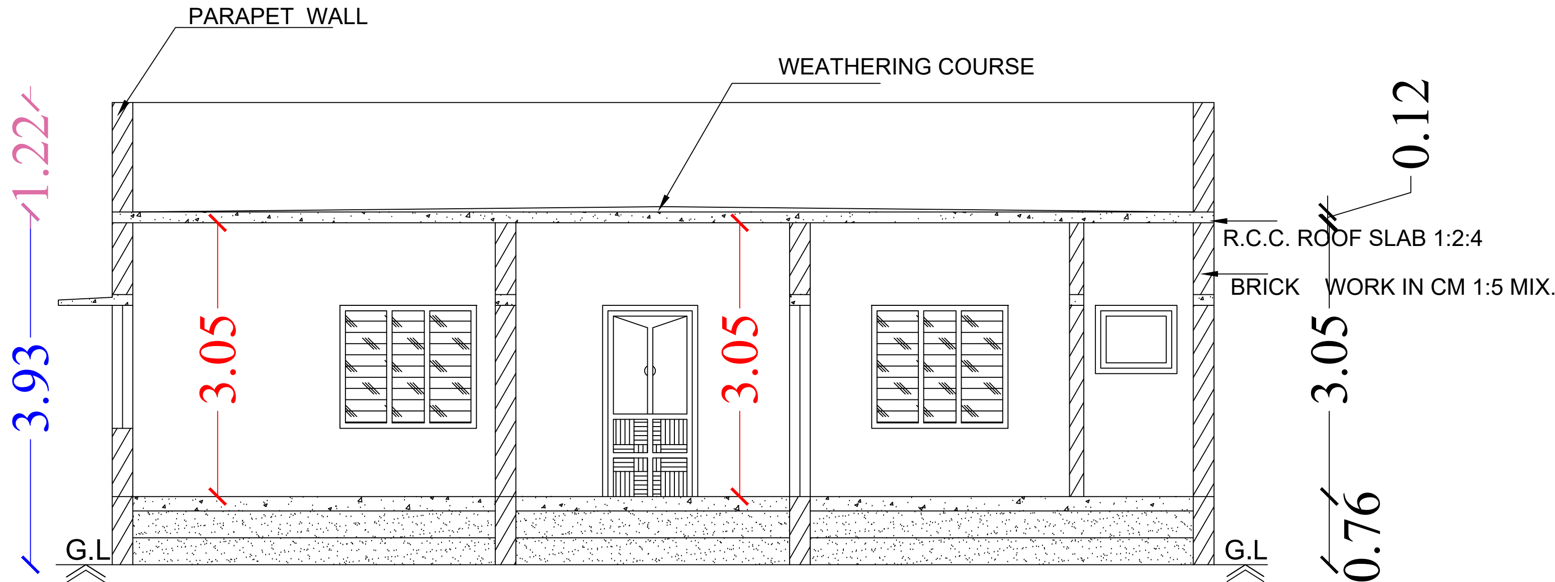
Section on-"AA"
