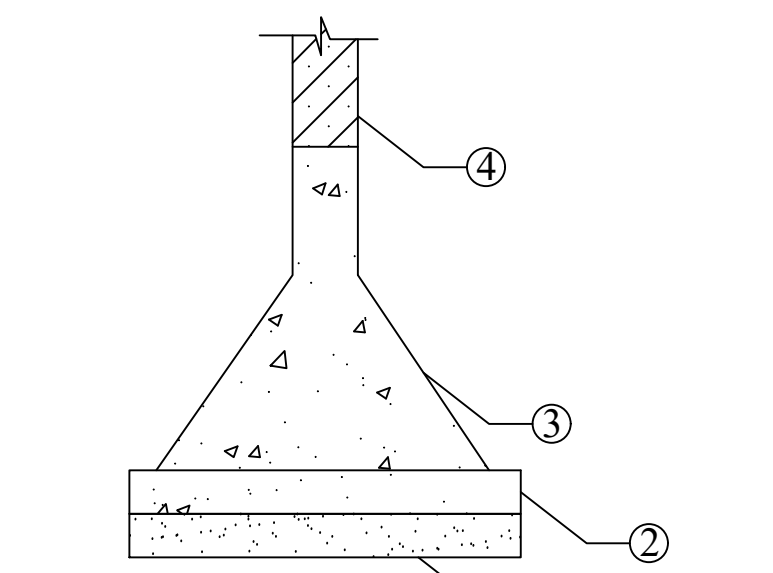
FOUNDATION DETAILS
