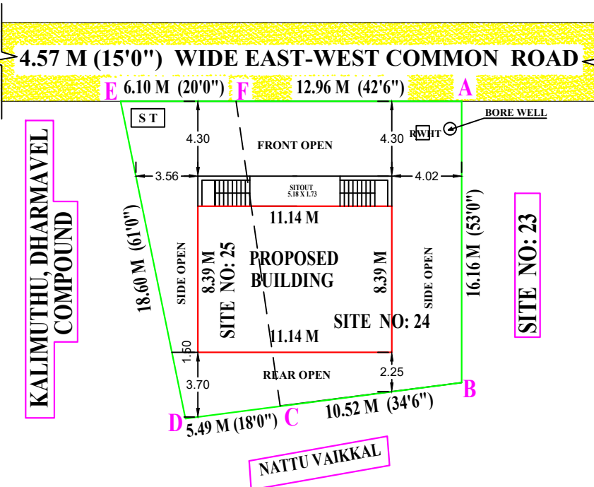
TOPO PLAN
