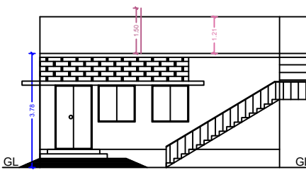
FRONT ELEVATION-2
