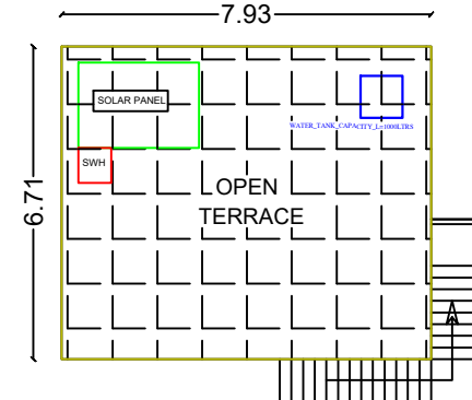
TERRACE FLOOR PLAN-2
