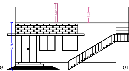
FRONT ELEVATION-1
