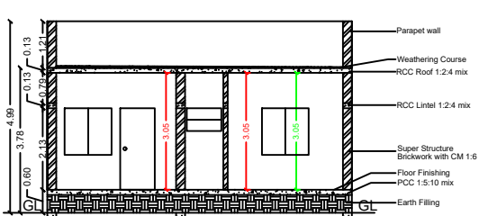
SECTION ON "VR"-1
