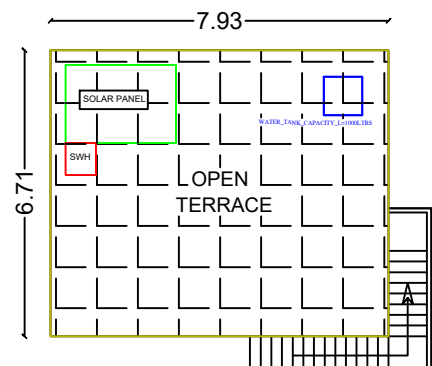
TERRACE FLOOR PLAN-1
