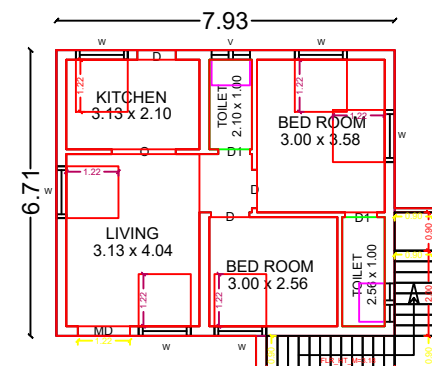
GROUND FLOOR PLAN-2
