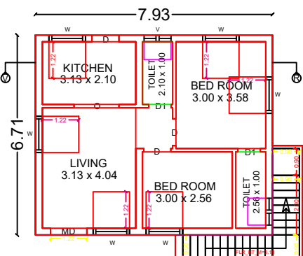
GROUND FLOOR PLAN-1
