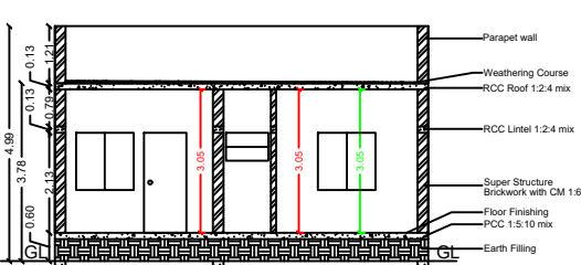
SECTION ON "VR"-2
