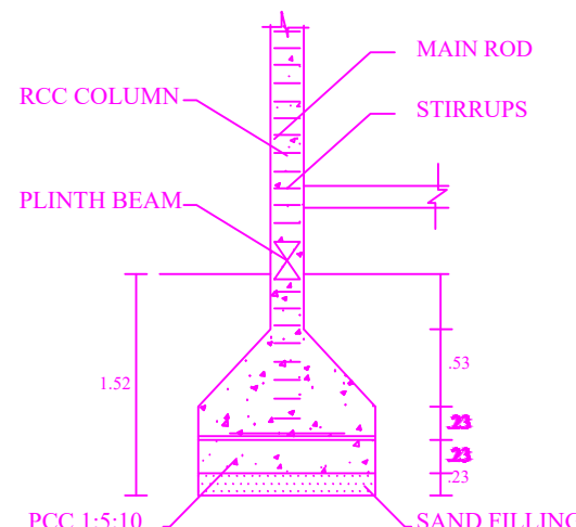
COLUMN DETAILS
