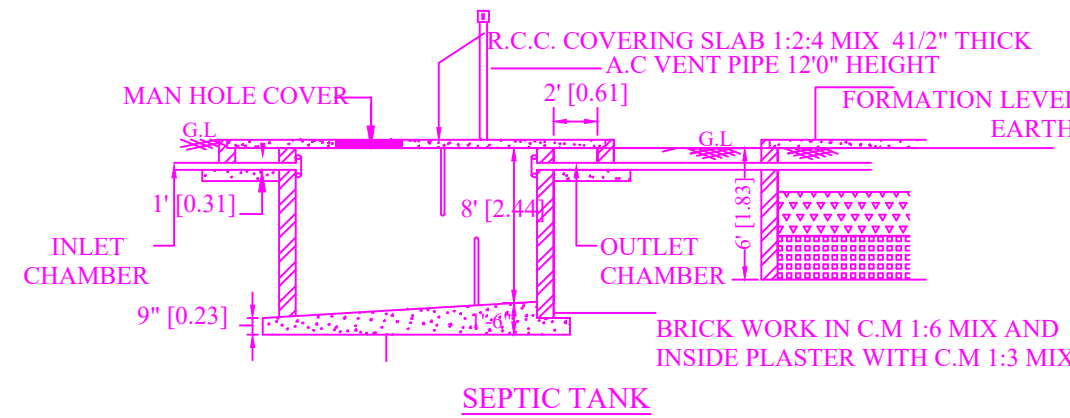
SEPTIC TANK
