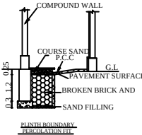
COMPOUND WALL
