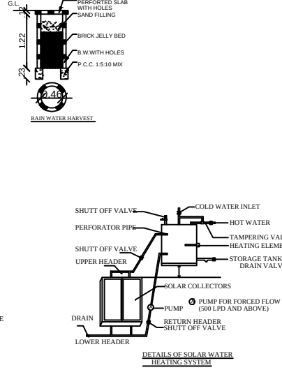
DETAILS OF SOLAR WATER HEATING SYSTEM
