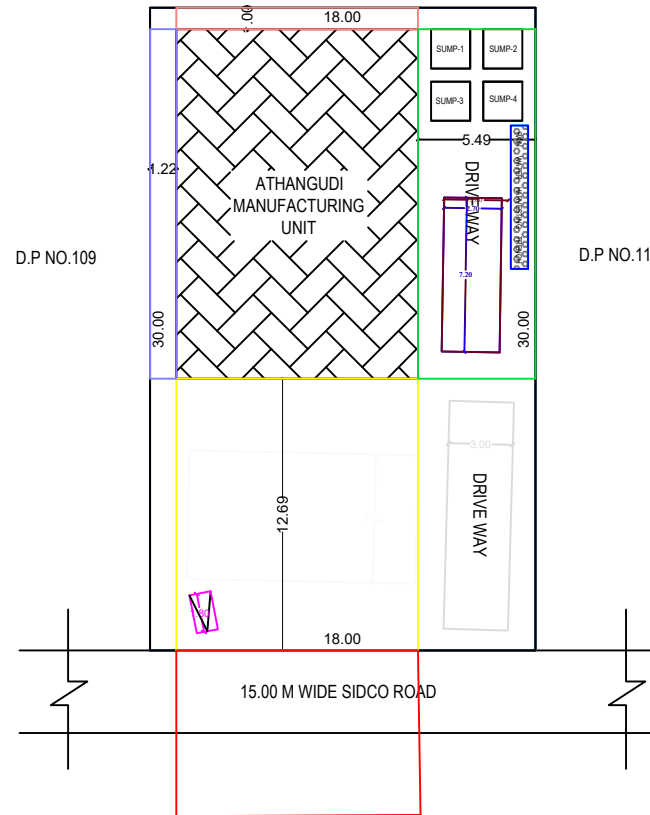
SIT PLAN (SCALE:1:200)
