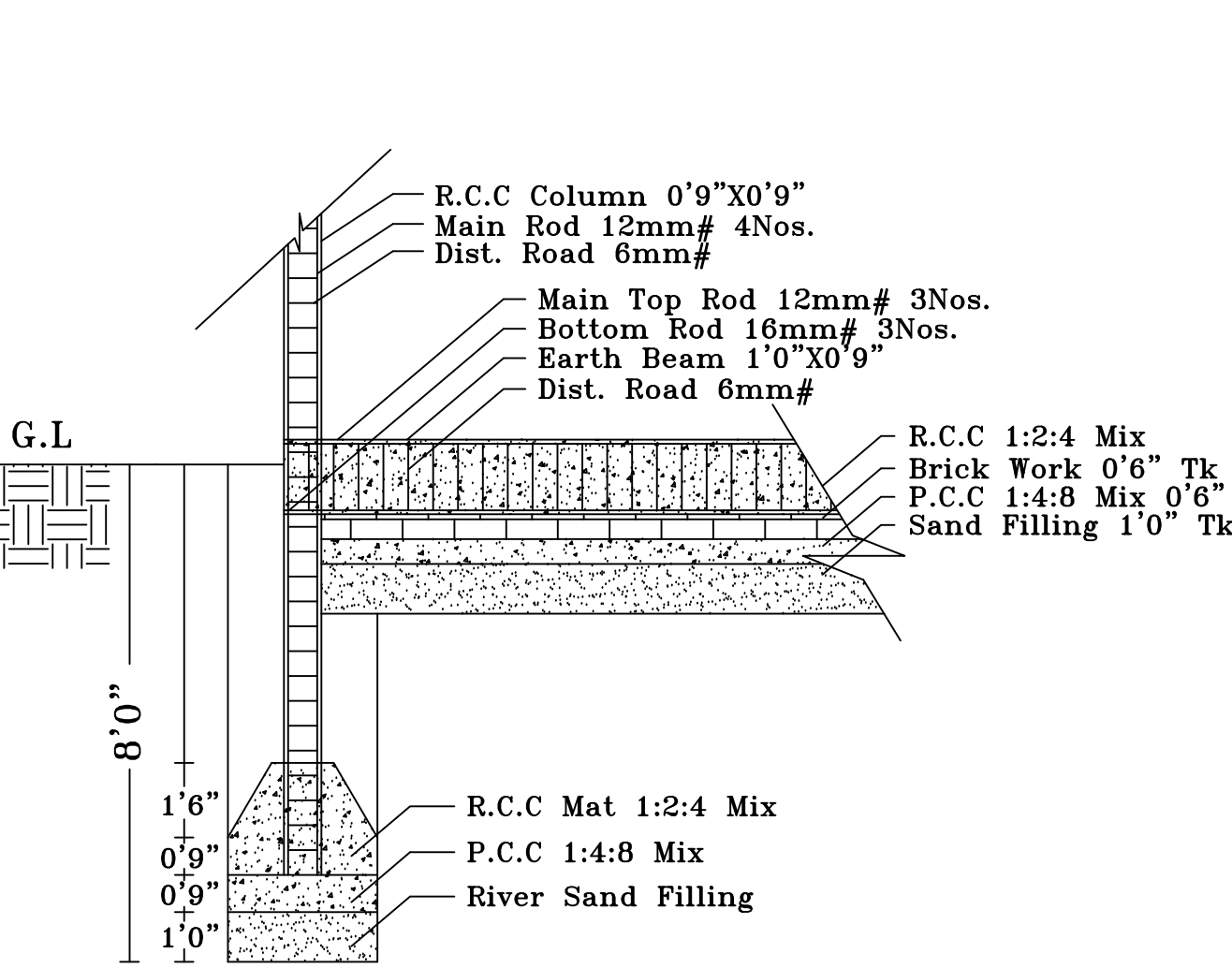
FOUNDATION DETAILS
