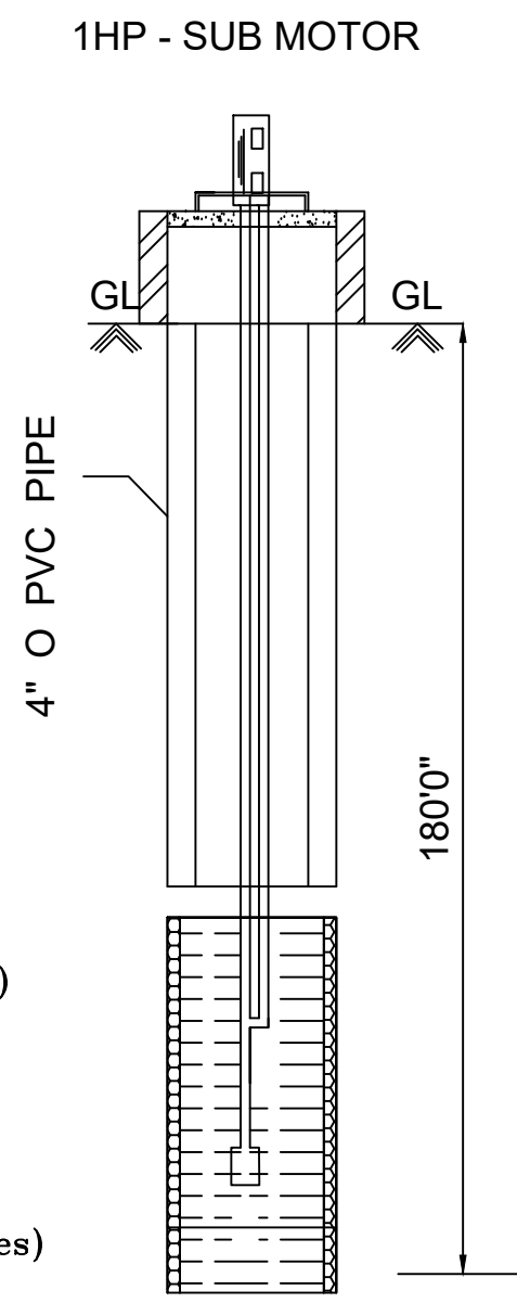
BORE WELL DETAILS
