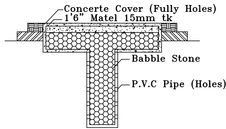
RAIN WATER STOREAGE TANK
