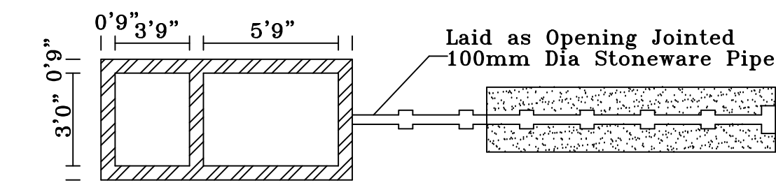
PLAN OF SEPTIC TANK
