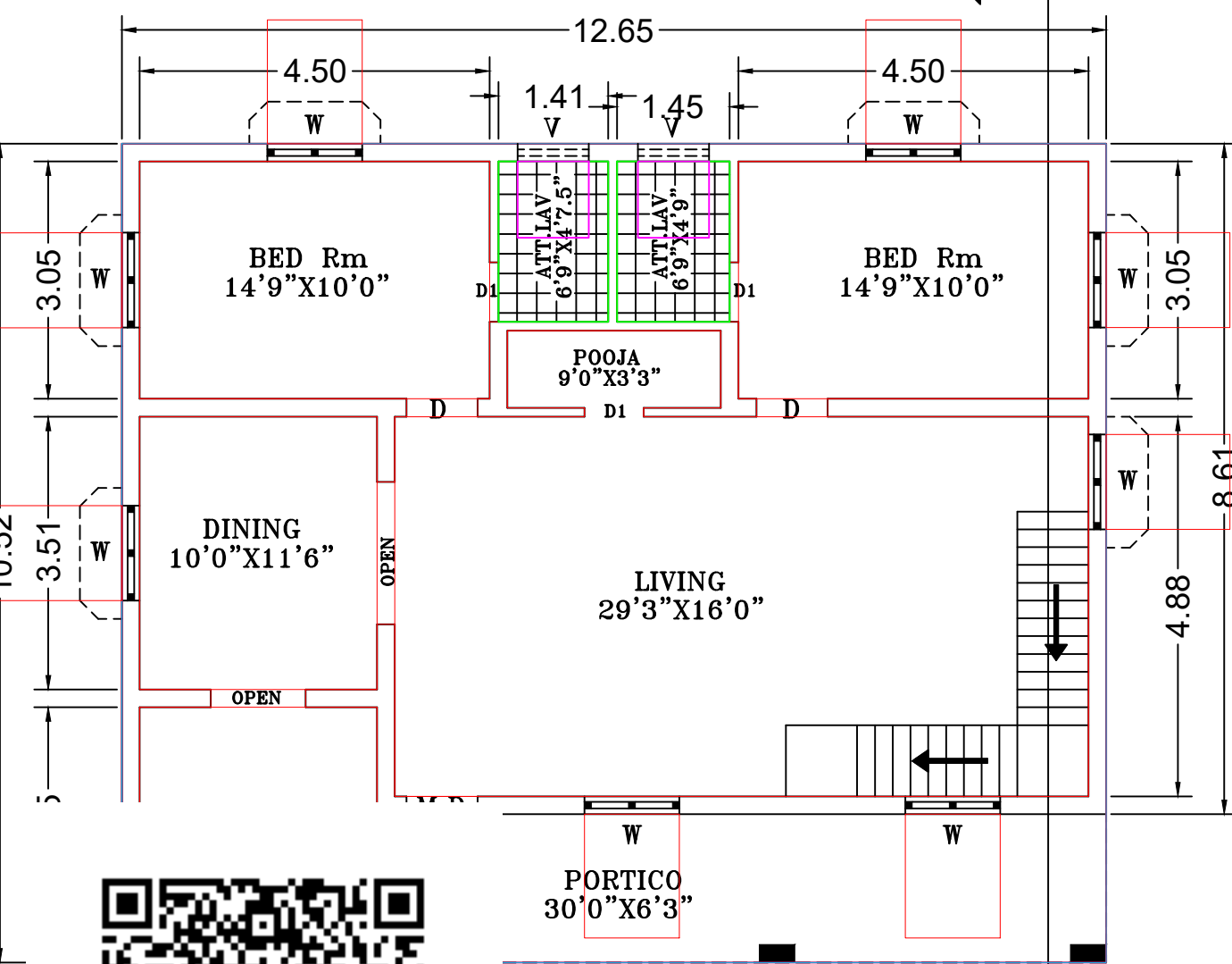
FLOOR PLAN
